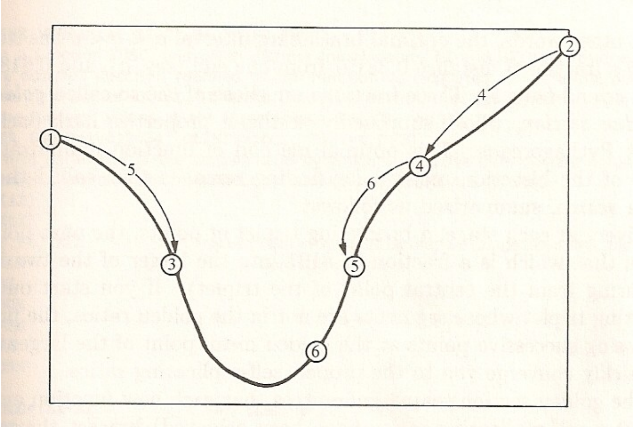
Figure 10.1.1. Successive bracketing of a minimum. The minimum is originally bracketed by points 1,3,2. The function is evaluated at 4, which replaces 2; then at 5, which replaces 1; then at 6, which replaces 4. The rule at each stage is to keep a center point that is lower than the two outside points. After the steps shown, the minimum is bracketed by points 3,6,5.
